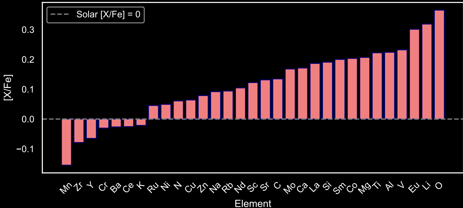
Abundance Pattern for GALAH Red Giants: Star Field [17] (N=64)
