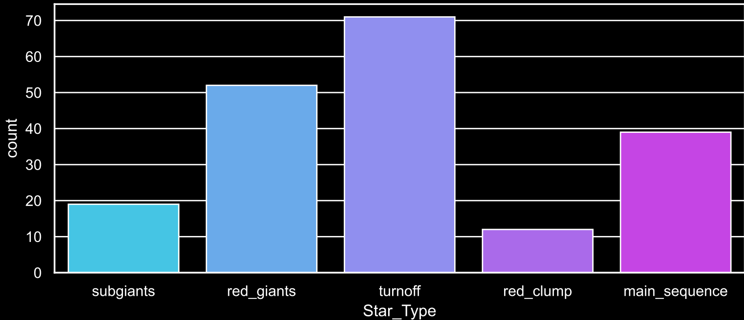
Field [17] Count plot of Star Type
