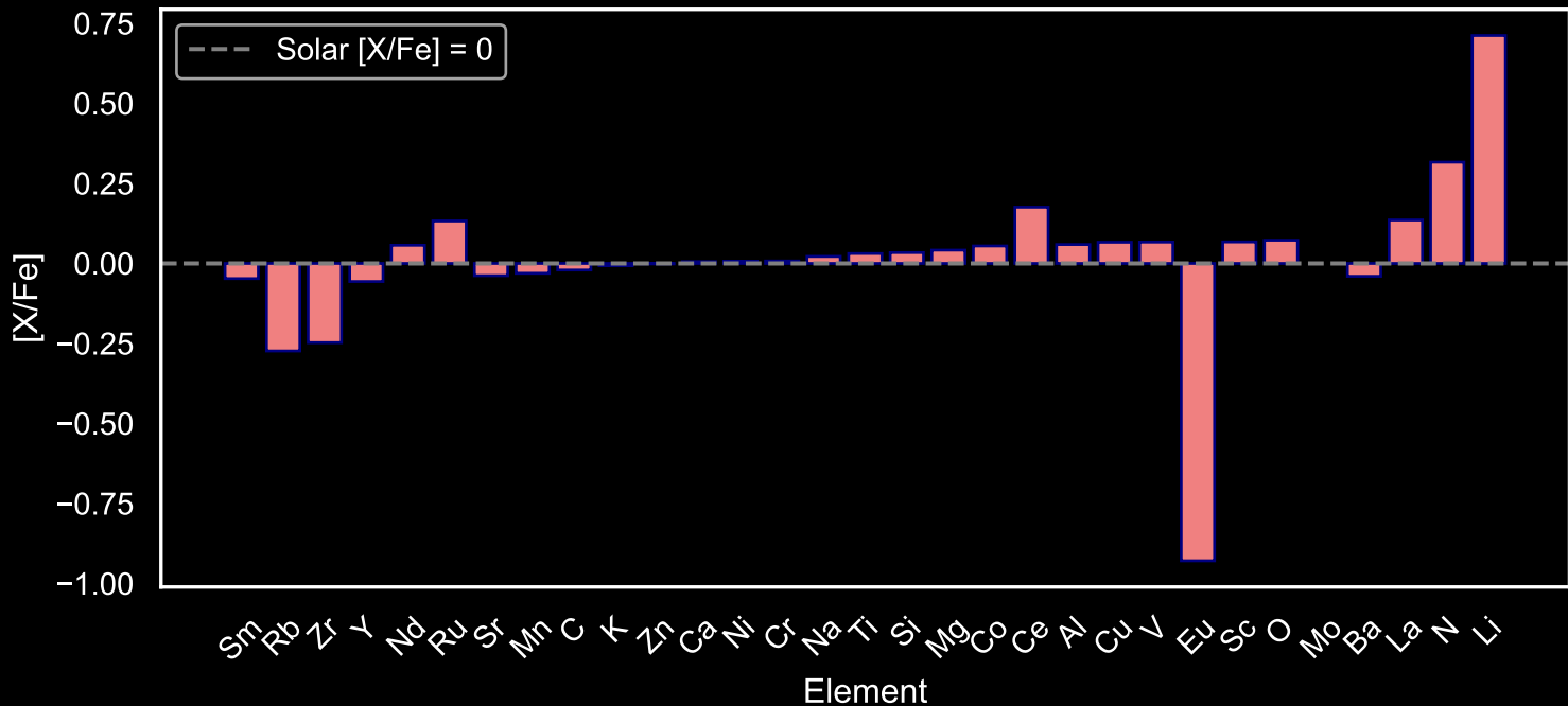
Abundance Pattern for GALAH Main Sequence Stars: Star Field [17] (N=39)
