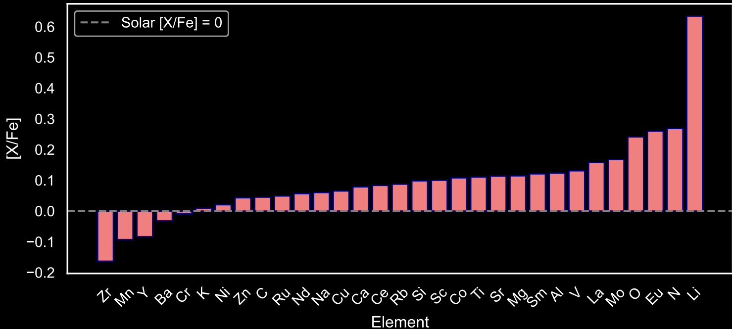
Abundance Pattern for GALAH Star Field [17] (N=193)
